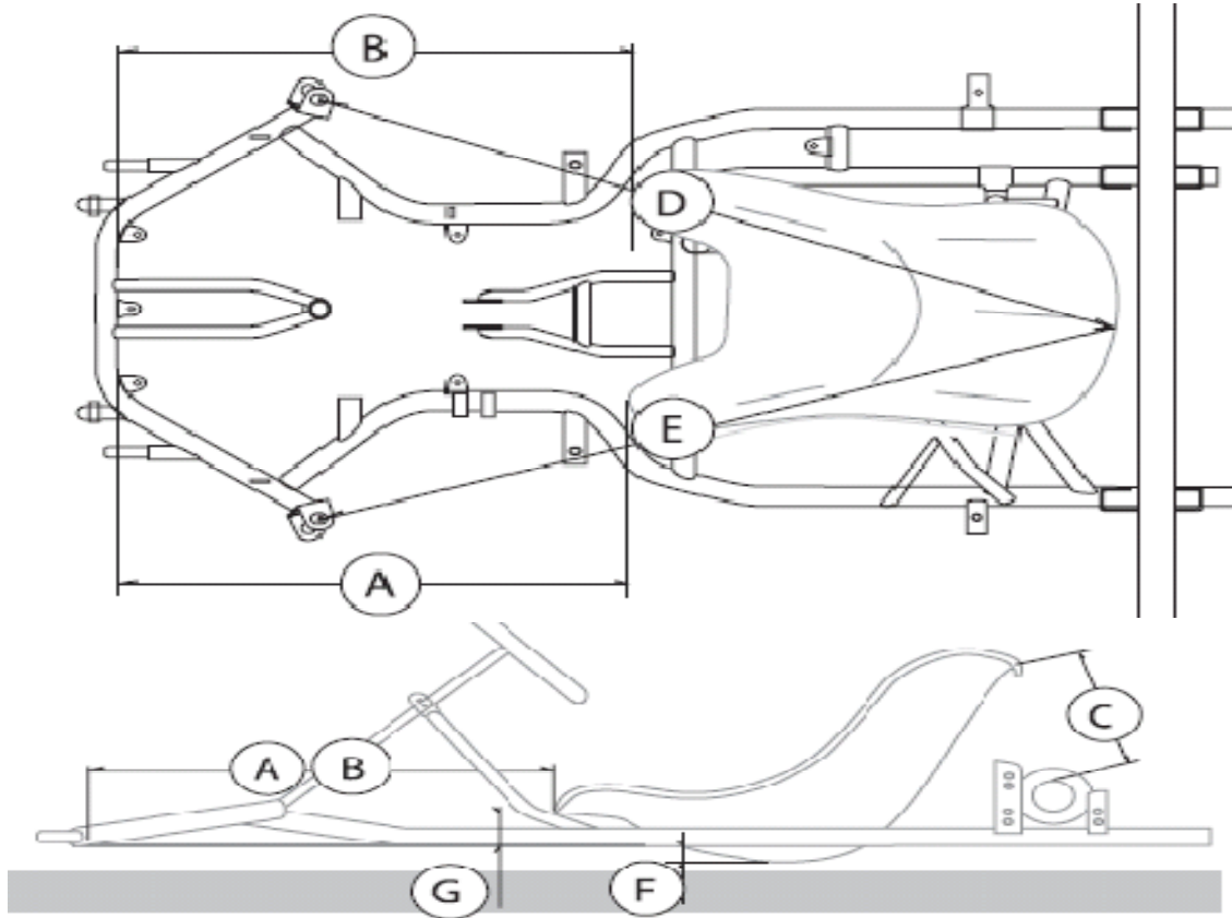
Dimensional Measurements
